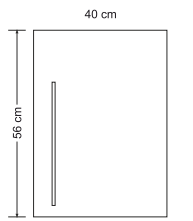
HS 40 - drawing
