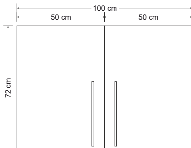
HS 100 - drawing
