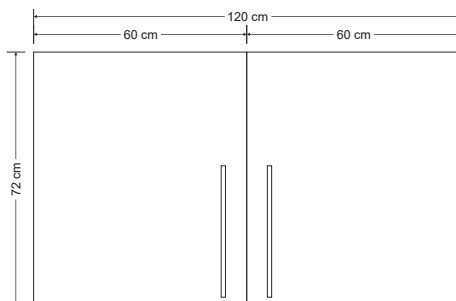
HS 120 - drawing
