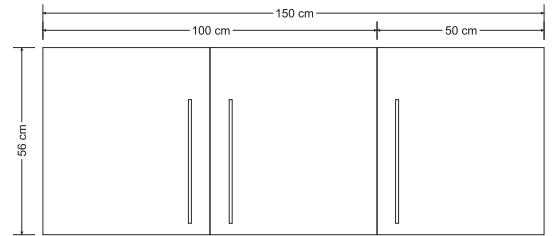
HS 150 - drawing
